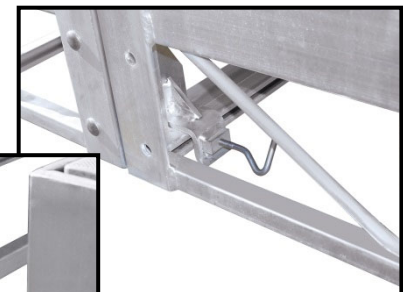
Single Stage Connection System
